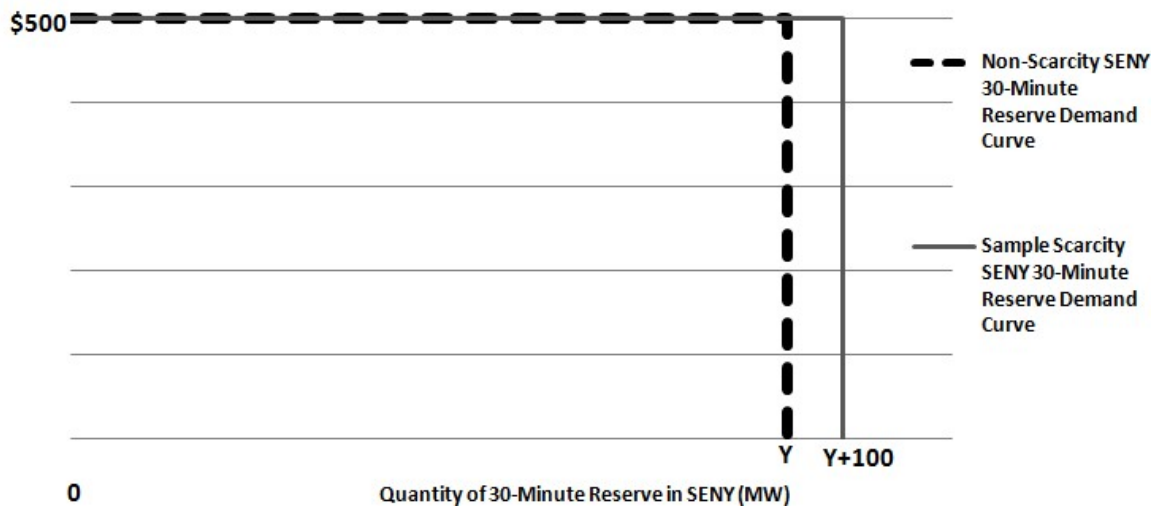
Example SENY 30-Minute Reserve Demand Curve during a Real-Time Interval in which a 100 MW Long Island Scarcity Reserve Requirement is Established
