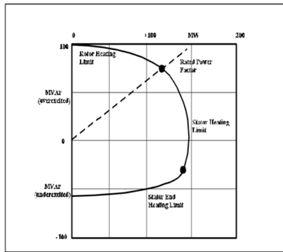
Figure 3: Generator MVAR versus MW Capability
